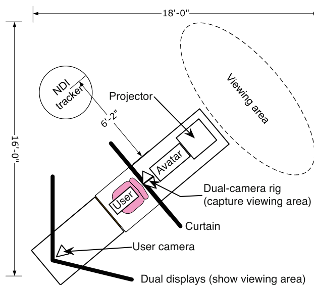
Fig. 4 Full-duplex configuration of the prototype system. The back-to-back setup was chosen to primarily to suit the capabilities of the NDI tracker while both presenting the Avatar to the viewers, and allowing the viewers to step to the side to see the human user/inhabiter
