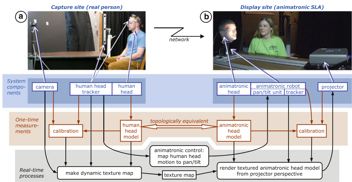
Fig. 2 Proof-of-concept implementation and diagram of Avatar user capture and display. At the capture site shown in (a), a camera captures a person, also tracked using a headband. At the display site shown in (b), a projector displays images onto an avatar consisting of
