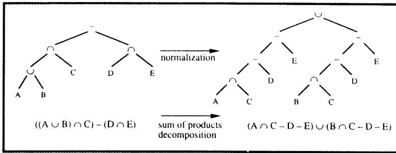
Figure 3. CSG tree before and after normalization.
