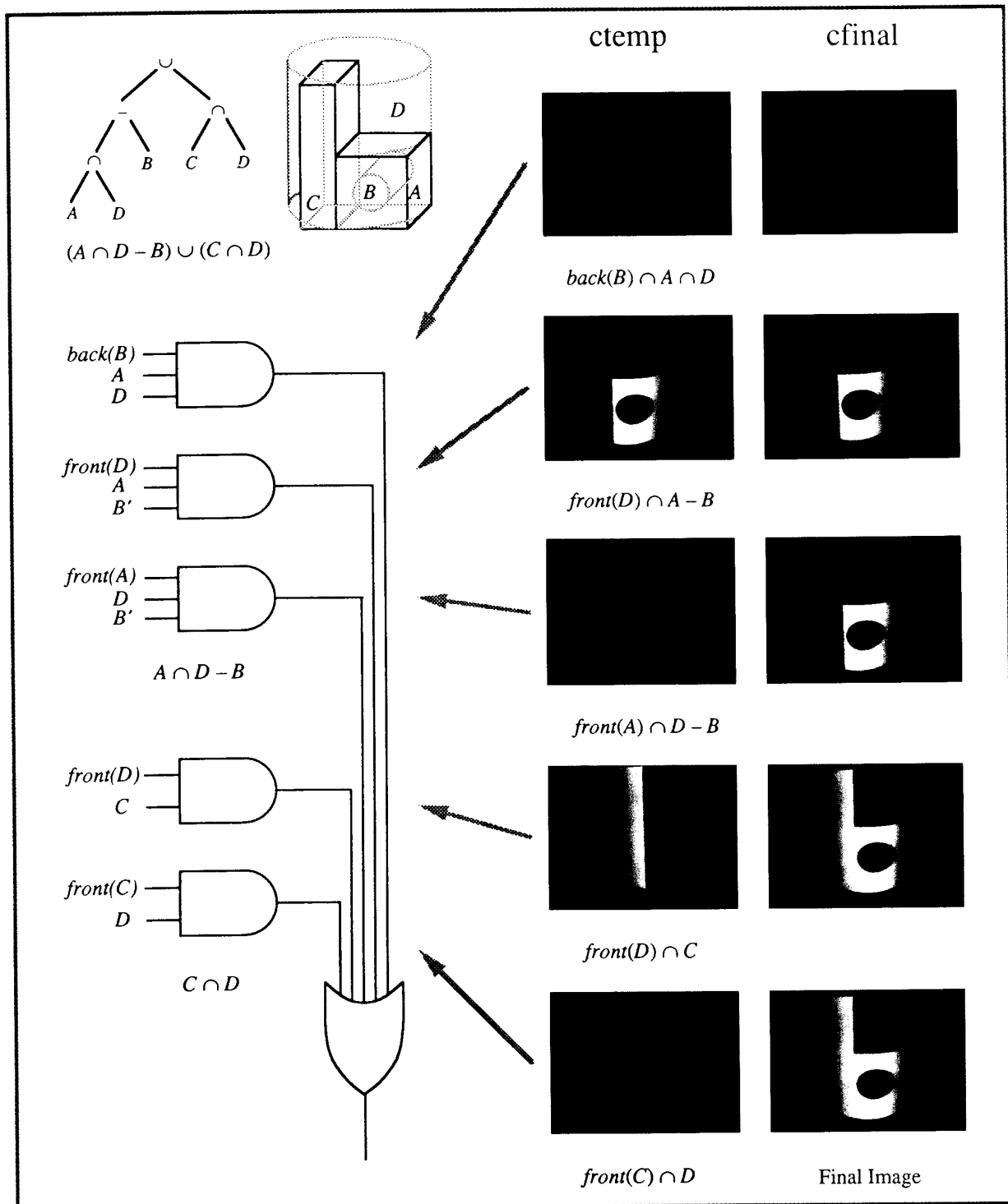
Figure 4. Rendering a CSG tree.
